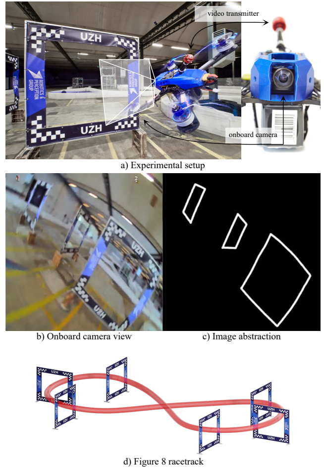
Fig. 1. Our autonomous quadrotor can fly through a racetrack purely based on images from an onboard camera, without explicit state estimation. a) overview of our experimental setup consisting of racing gates, a quadrotor equipped with an onboard camera, and a video transmitter, b) onboard view from the camera, c) image abstraction used by the policy, d) overview over the racetrack.
